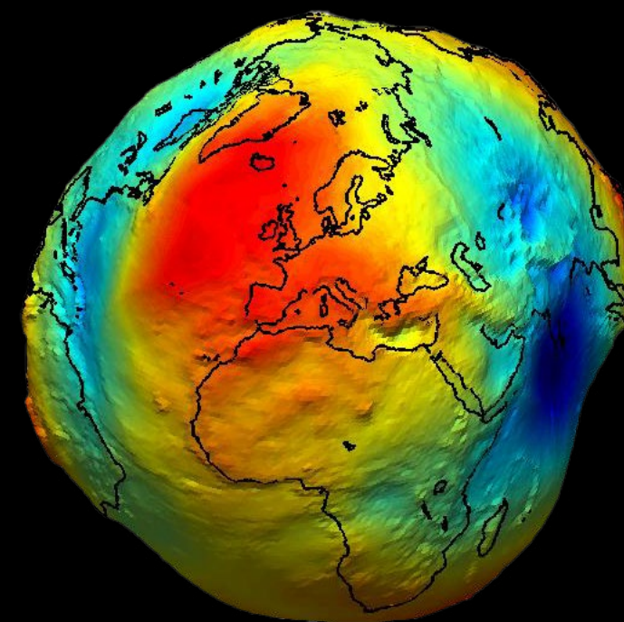
VLBI measurements of distant ‘static’ radio sources help define the Earth's exact shape and rotation speed. Credit: ESA
